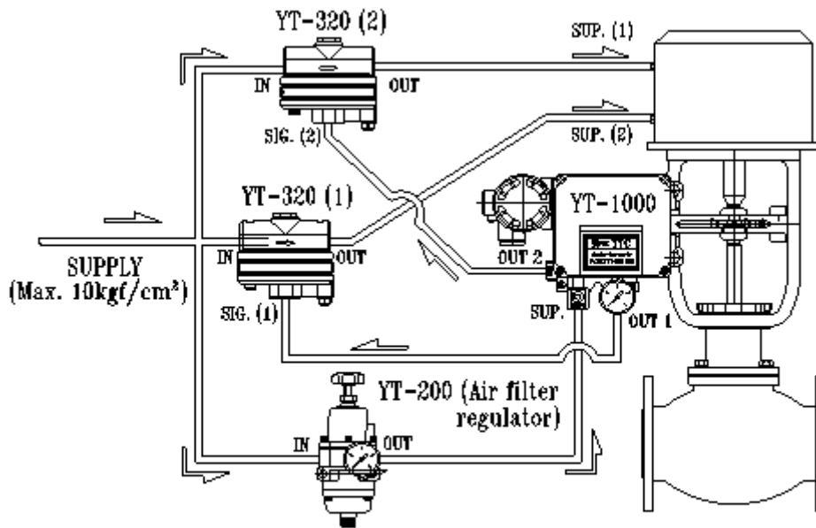
LINEAR ACTUATOR TYPE
